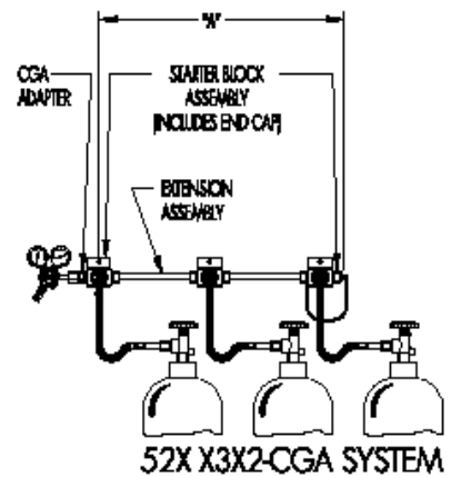
Regulator System
