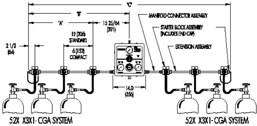
Switchover System
