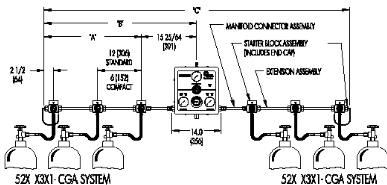
Switchover System
