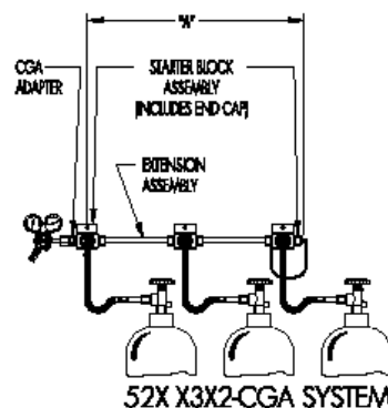
Regulator System
